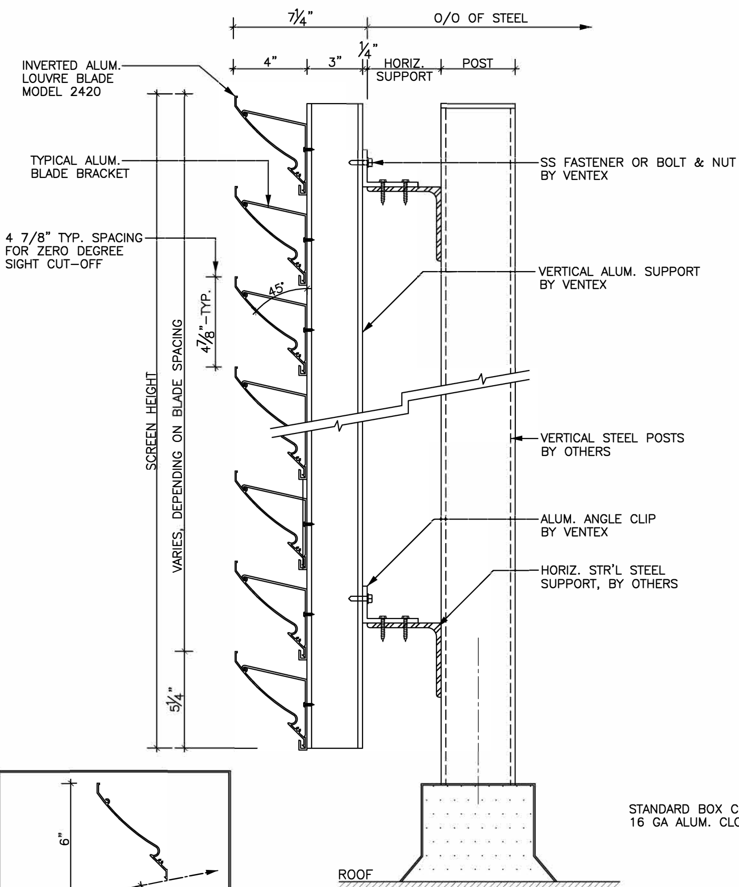
VERT. SECTION TYP. SCALE: 3/16"=1"
